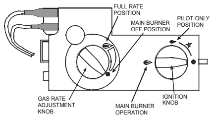
Figure 7 – Gas Valve
