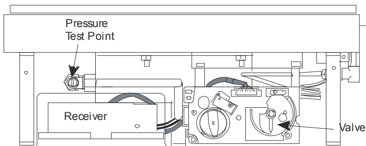
Figure 51 - Total Control Model
