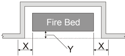
X=150mm, less dimension Y Figure 57
