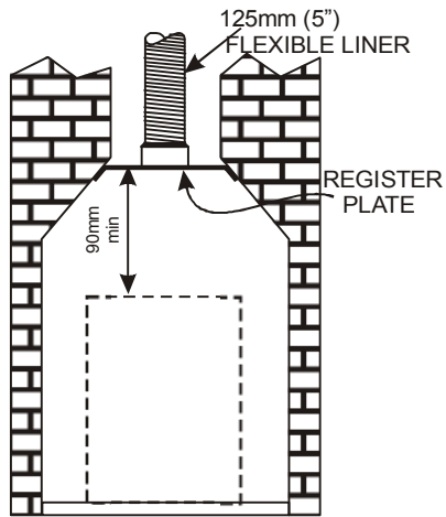
SECTION THROUGH MASONRY CHIMNEY Figure 45
