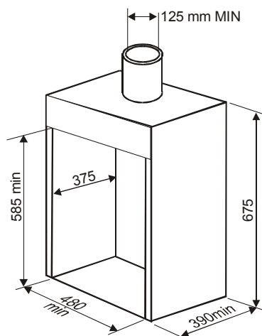
Figure 44 – Minimum Dimensions of Metal Flue Box
