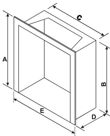
Figure 47 - Thermobox Dimensions
