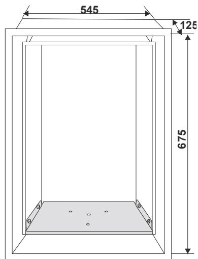
Figure 48- Freedom Frame Dimensions
