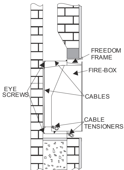
Figure 66 – Freedom Frame Installation with firebox fitted
