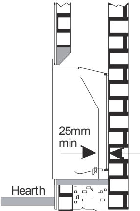
Figure 53 - Catchment Space
