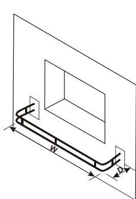
Figure 59 – Example of physical barrier (dimensions as stated in Table 4 – Protected Area)
