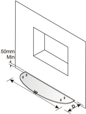
Figure 61 – Example of physical barrier (dimensions as stated in Table 4 – Protected Area)
