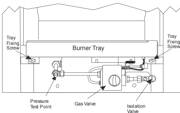
Figure 48 – Ekos 16'' with BM Valve
