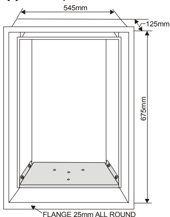
Figure 67 - General Dimensions
