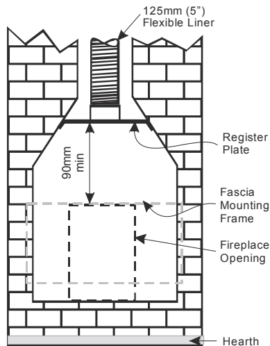
Figure 46 – Section through Masonry Chimney
