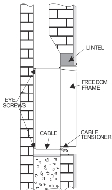
Figure 65 – Freedom Frame Installation in Conventional Chimney
