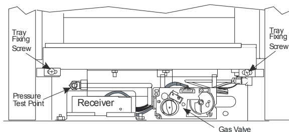
Figure 50 - Ekos 16" with Mertik GV60 Valve (Total Control)
