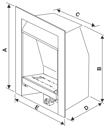
Figure 47 - Standard Box Dimension (refer to Table 1)
