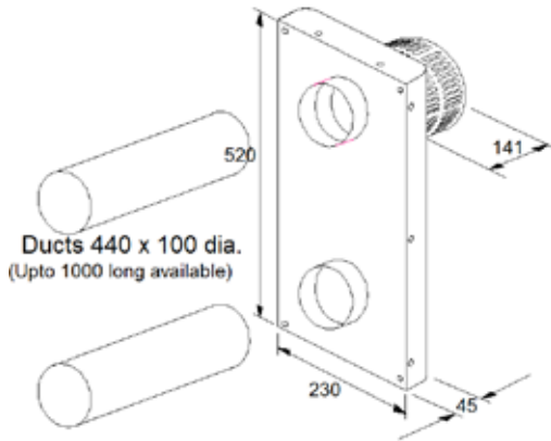
FIGURE 11 Flue Pipe and Air Box with terminal (all dimensions in mm)
